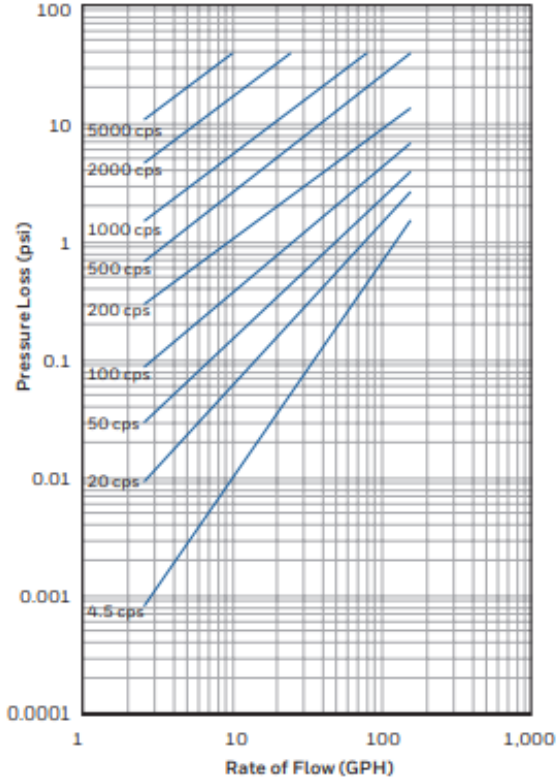
Controls Warehouse CW15—1/2" Fuel Oil Meter
