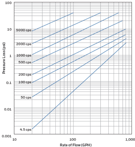
Controls Warehouse CW25—1" Fuel Oil Meter
