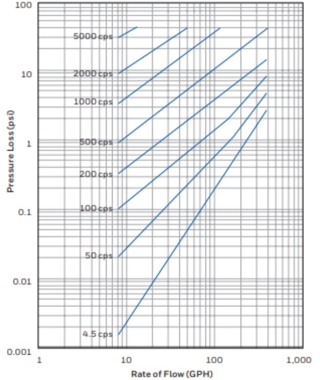
Controls Warehouse CW20—3/4" Fuel Oil Meter
